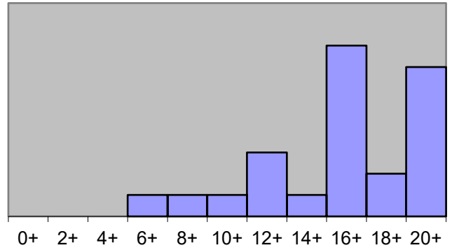
Problem #2 Scores
