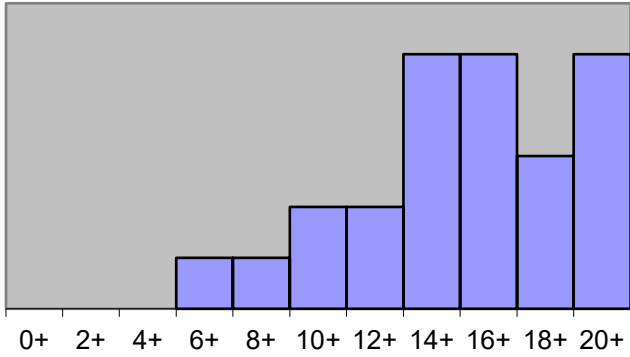
Problem #3 Scores
