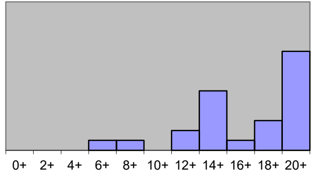
Problem #6 Scores
