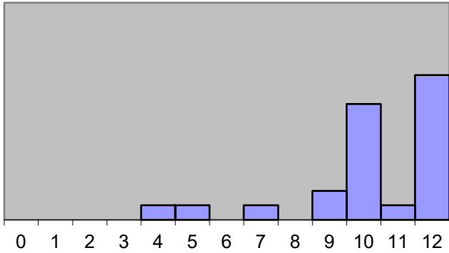
Problem #5 Scores
