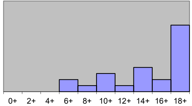
Problem #4 Scores
