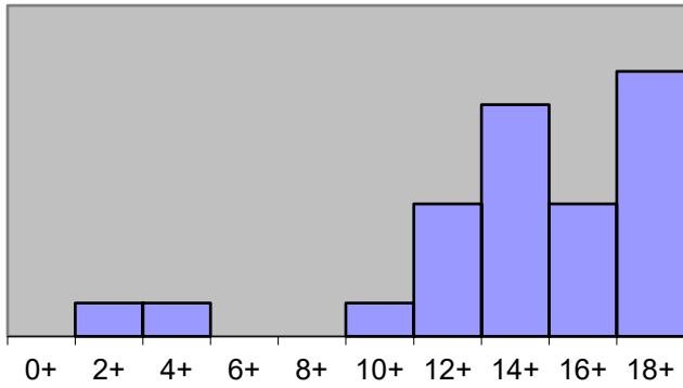
Problem #5 Scores
