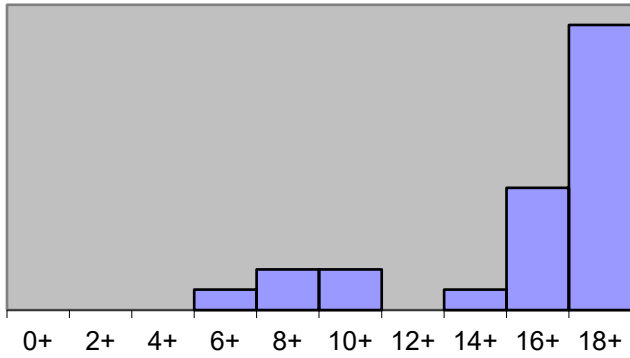
Problem #3 Scores
