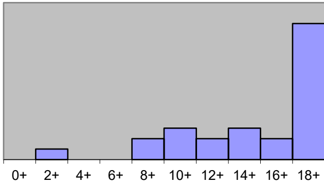
Problem #1 Scores
