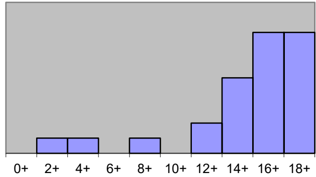
Problem #4 Scores
