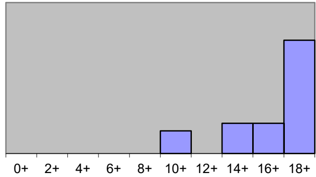
Problem #2 Scores
