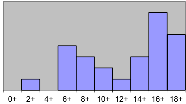
Problem #6 Scores
